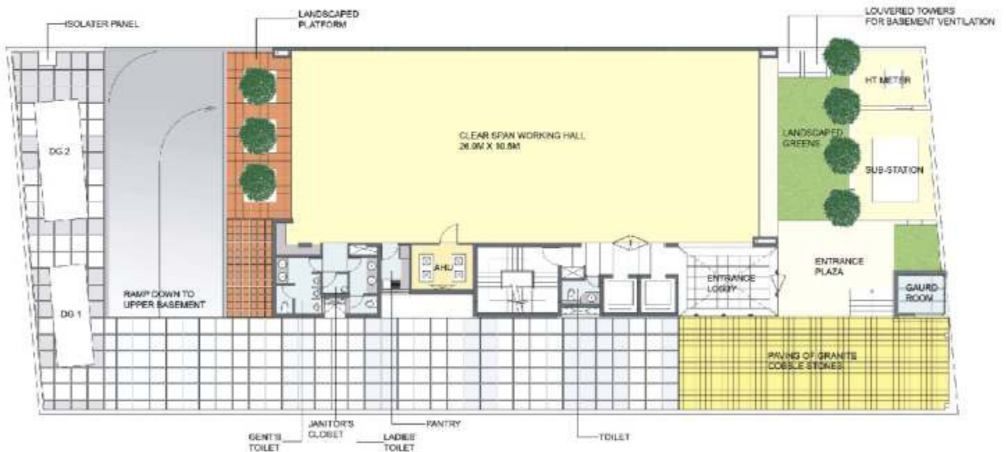
Typical Floor Plan : 416sq.m. approx.
